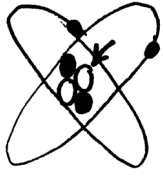
neutron
